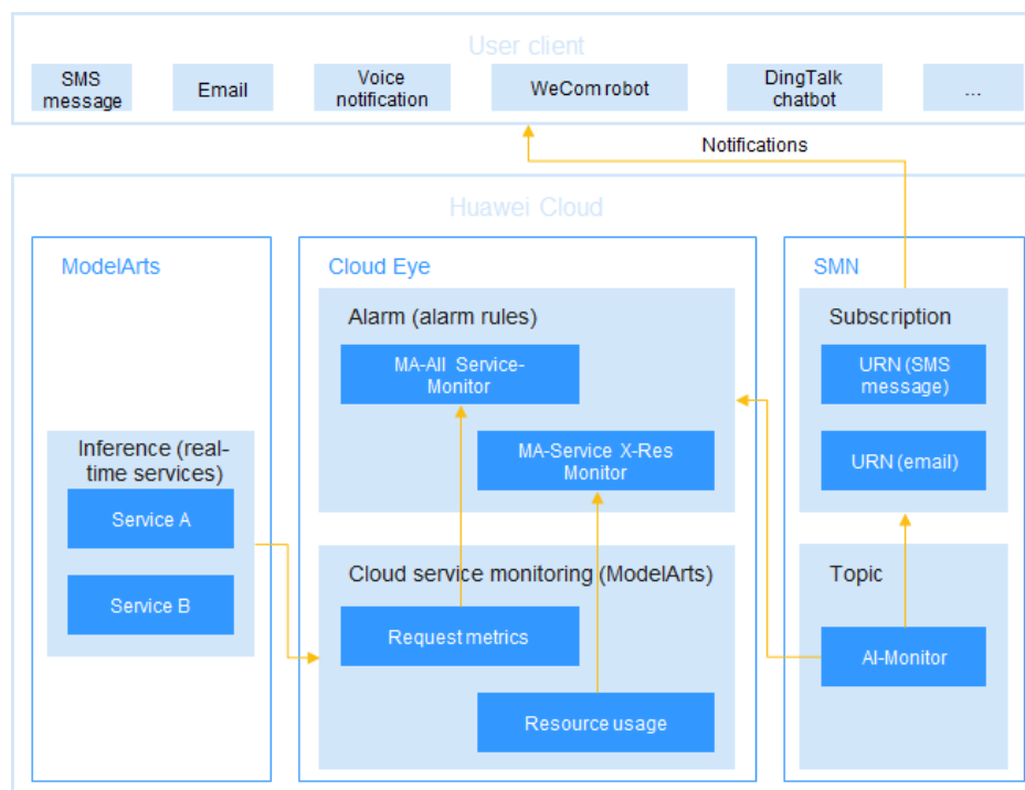
Figure 2-27 Alarming process
