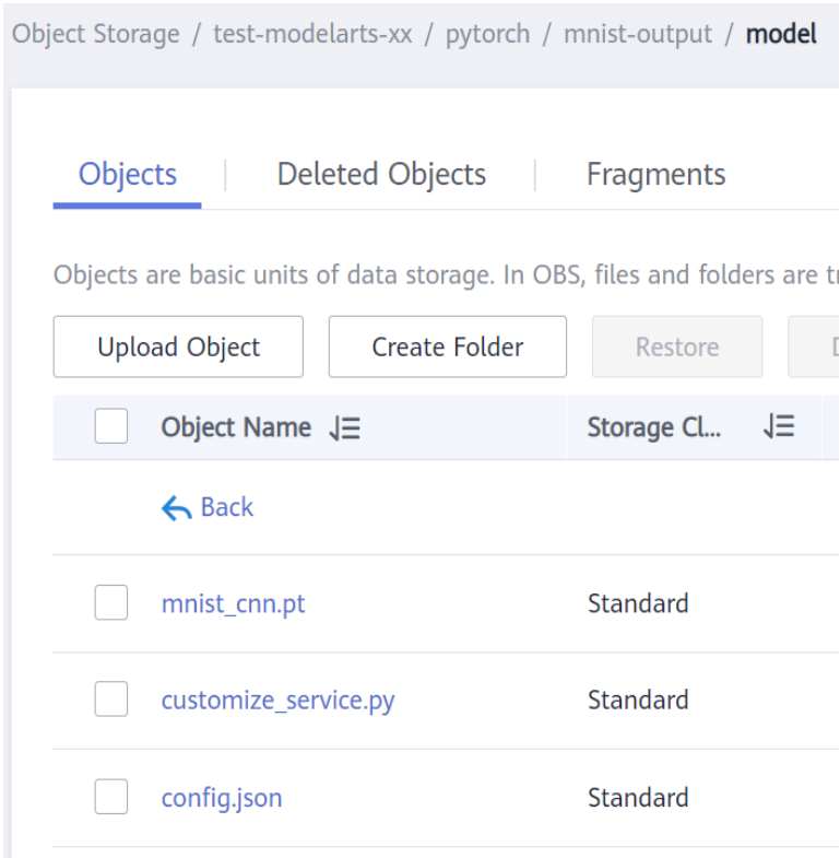
Figure 2-13 Trained model
