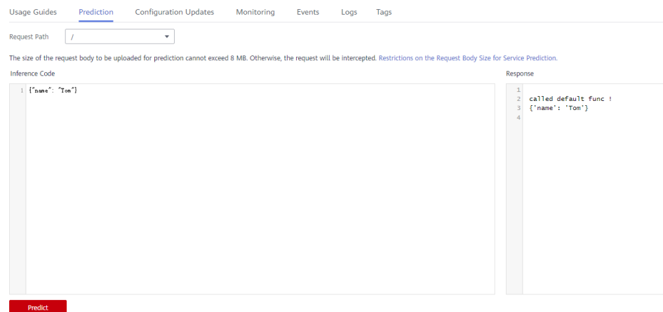
Figure 2-34 Prediction
